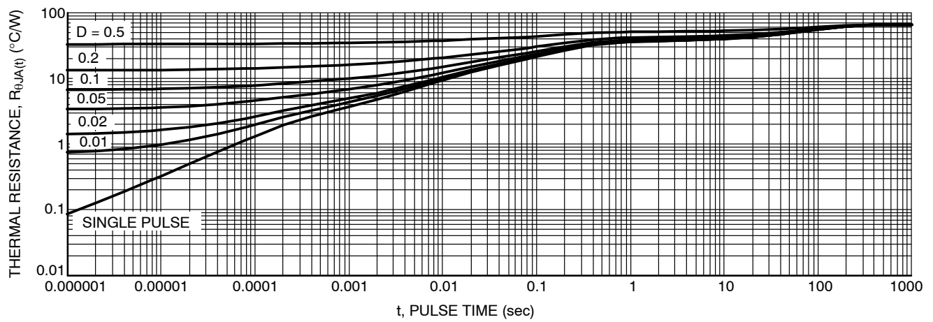
Figure 26. Thermal Response
