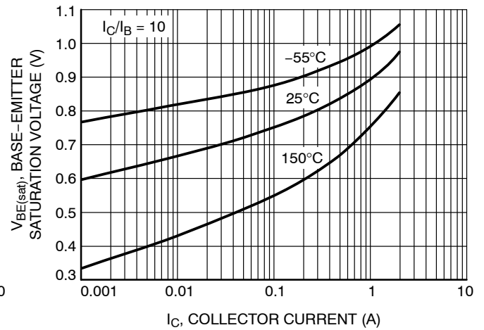
Figure 4. Base Emitter Saturation Voltage vs. Collector Current
