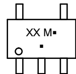
SC-88A CASE 419A
