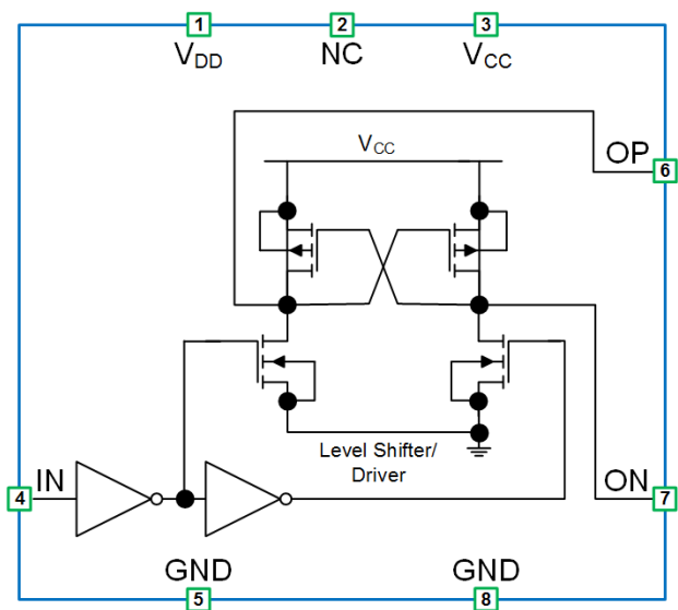
Figure 1. Block Diagram
