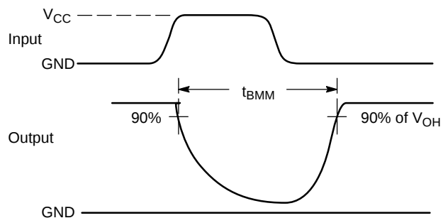
Figure 2. t_{\text{BBM}} (Time Break-Before-Make)
