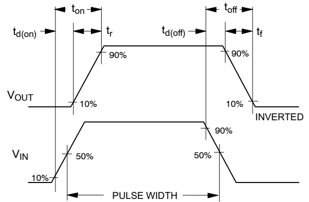
Figure 12. Switching Waveforms
