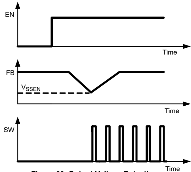
Figure 29. Output Voltage Detection
