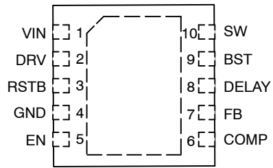
Figure 3. Pin Connections
