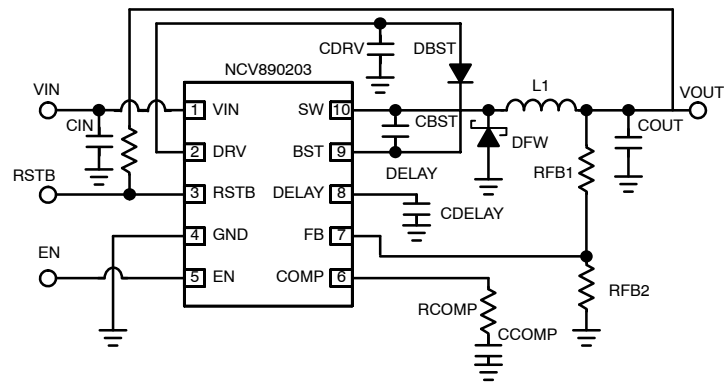
Figure 1. Typical Application
