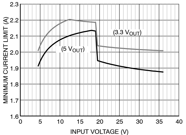
Figure 26. NCV890203 Load Current Capability with 4.7 \mu H Inductor
