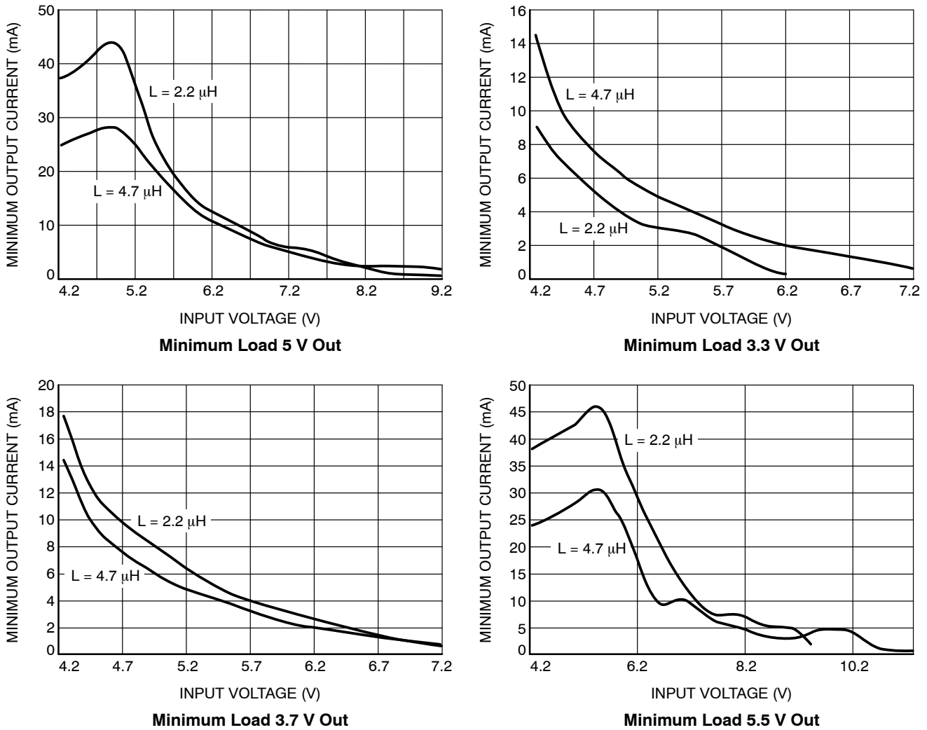
Figure 28. Minimum Load Current with Different Input and Output Voltages
