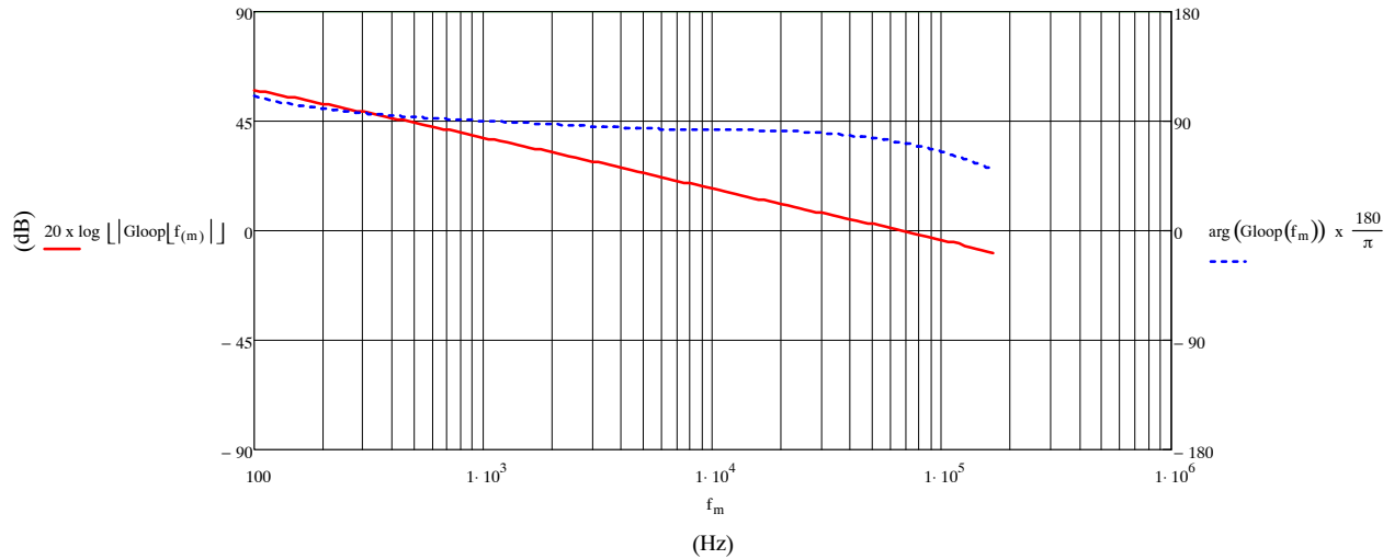
Figure 34. Bode Plot of the Total Loop
