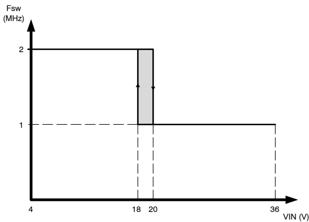
Figure 25. NCV890203 Switching Frequency Reduction at High Input Voltage
