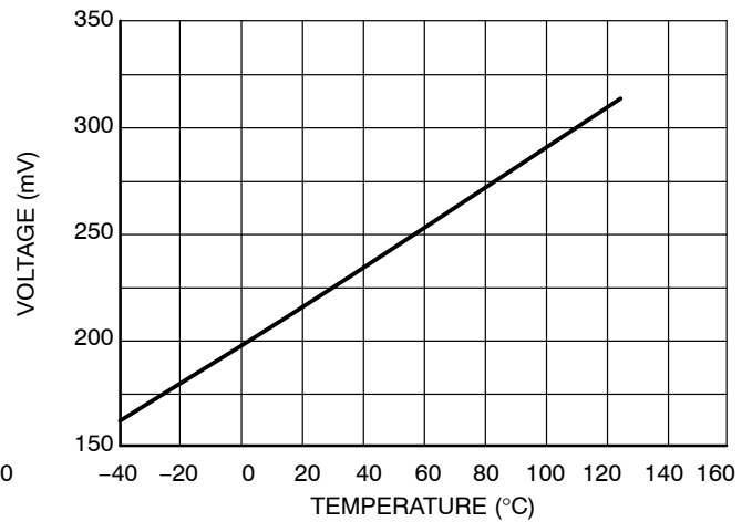
Figure 14. 5P0 Dropout Voltage Limit vs. Temperature
