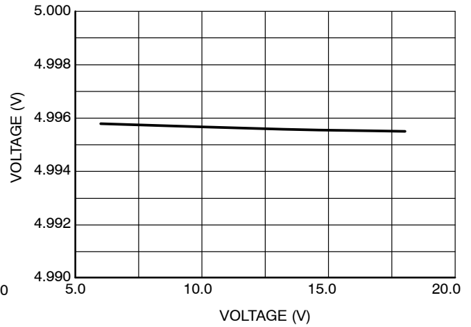
Figure 12. 5P0 Output Voltage vs. Input Voltage
