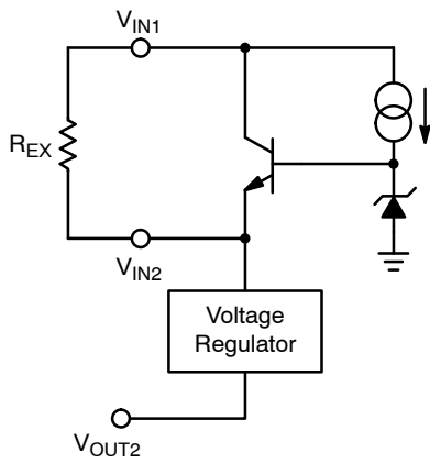
Figure 42. Power Shunt
