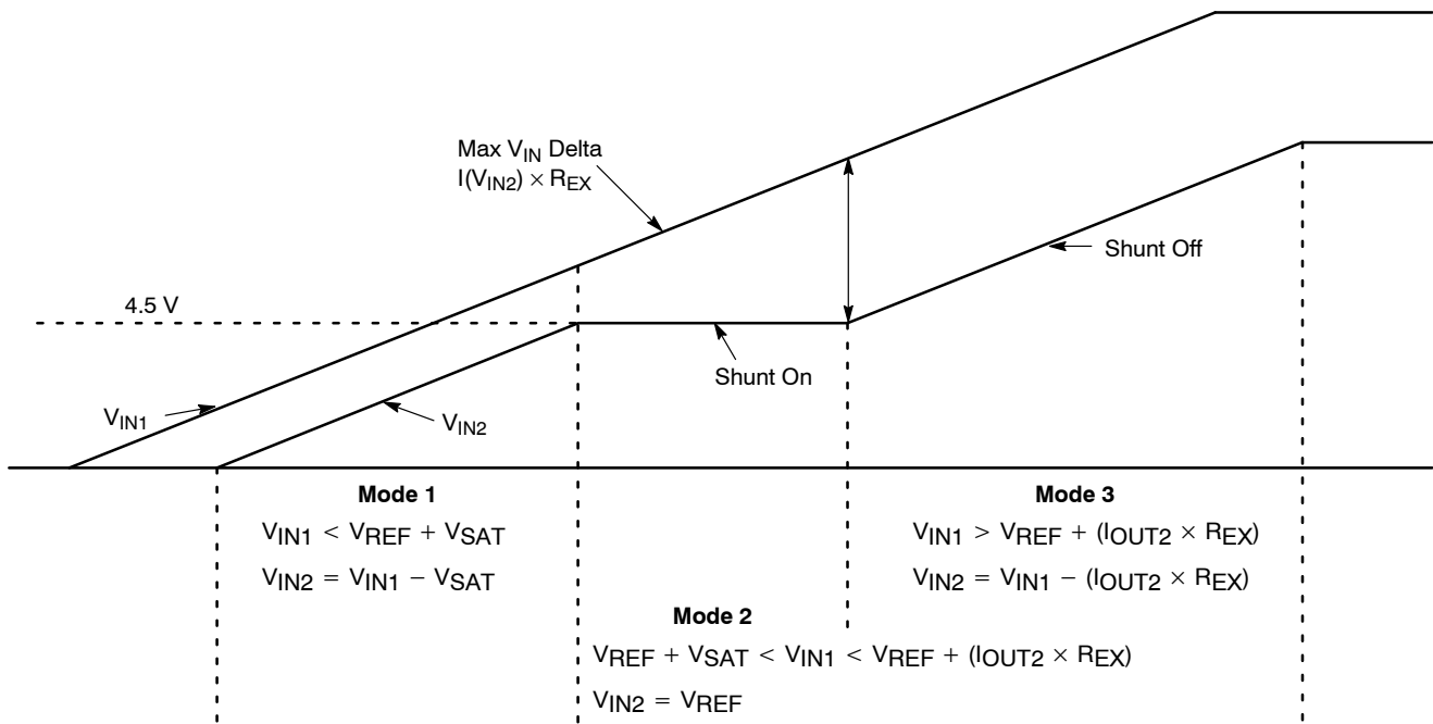
Figure 50. V_{IN} Shunt
