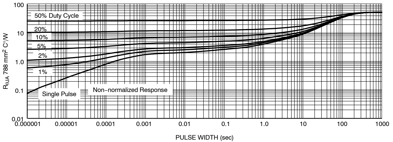
Figure 23. Duty Cycle for 1" Spreaders Boards, D 2 PAK 5-Lead
