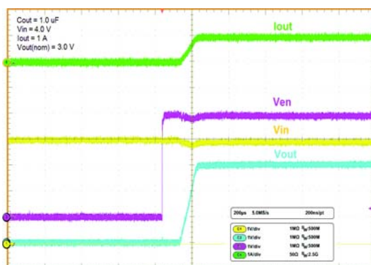
Figure 36. Turn-on by Enable Signal
