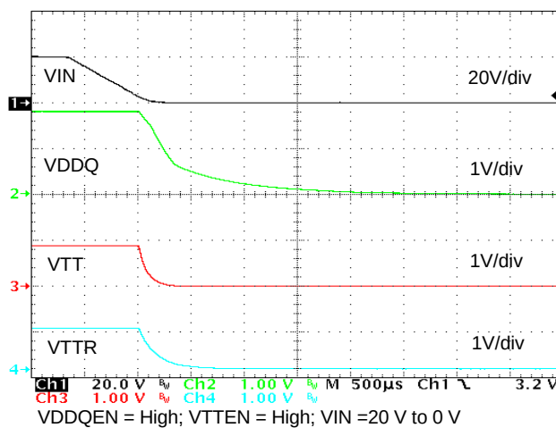
Figure 18. Power-Down Waveforms
