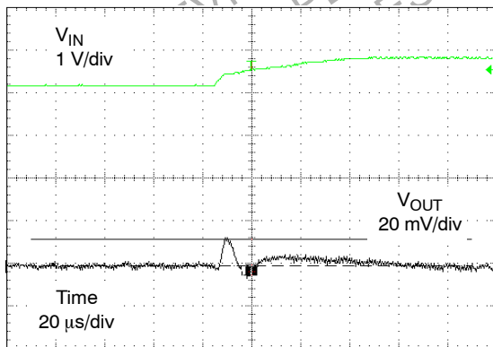
Figure 17. 3.0 V to 3.6 V Line Transient (Risetime = 50 \mu\text{s} , V_{OUT} = 1.2 \text{ V} , I_{OUT} = 100 \text{ mA} , T_A = 25^\circ\text{C} )
