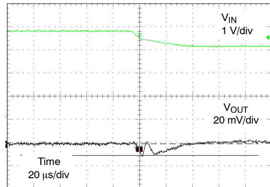
Figure 18. 3.6 V to 3.0 V Line Transient (Risetime = 50 \mu\text{s} , V_{OUT} = 1.2 \text{ V} , I_{OUT} = 100 \text{ mA} , T_A = 25^\circ\text{C} )
