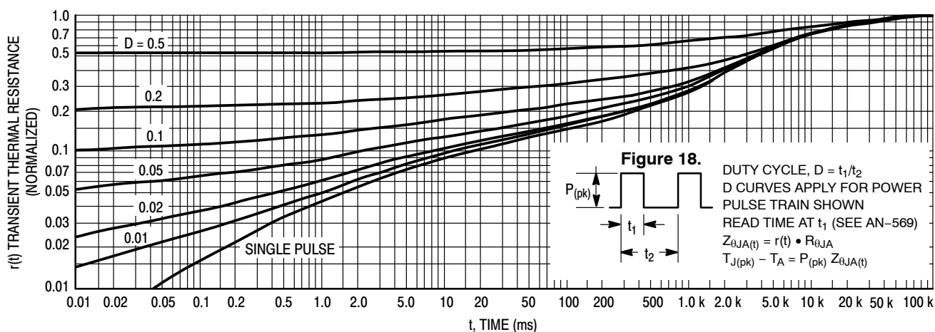
Figure 17. Thermal Response
