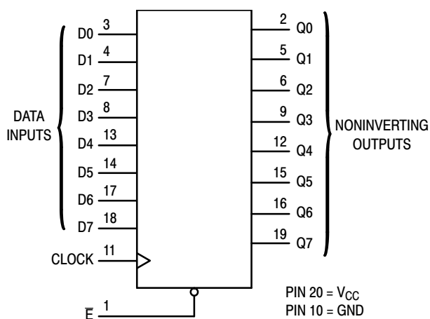
Figure 1. Logic Diagram
