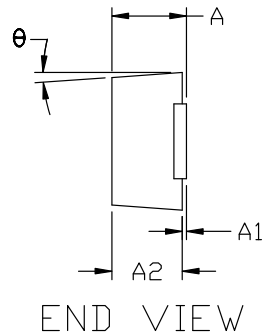
SOD-123-2 1.65x2.70x0.90 CASE 498 ISSUE E
