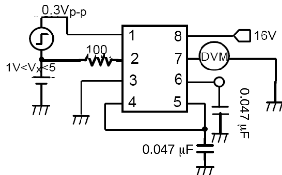
Figure 18. Response Time
