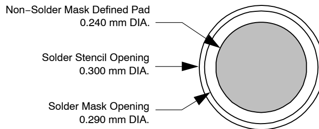
Figure 6. Recommended Non-Solder Mask Defined Pad Illustration
