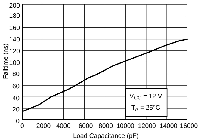
Figure 5. GATE(H) &amp; GATE(L) Falltime vs. Load Capacitance
