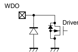
Equivalent Circuit for WDO Pin (R5115xxx2C)
