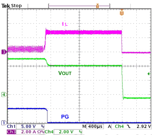
Figure 19. Overload Protection
