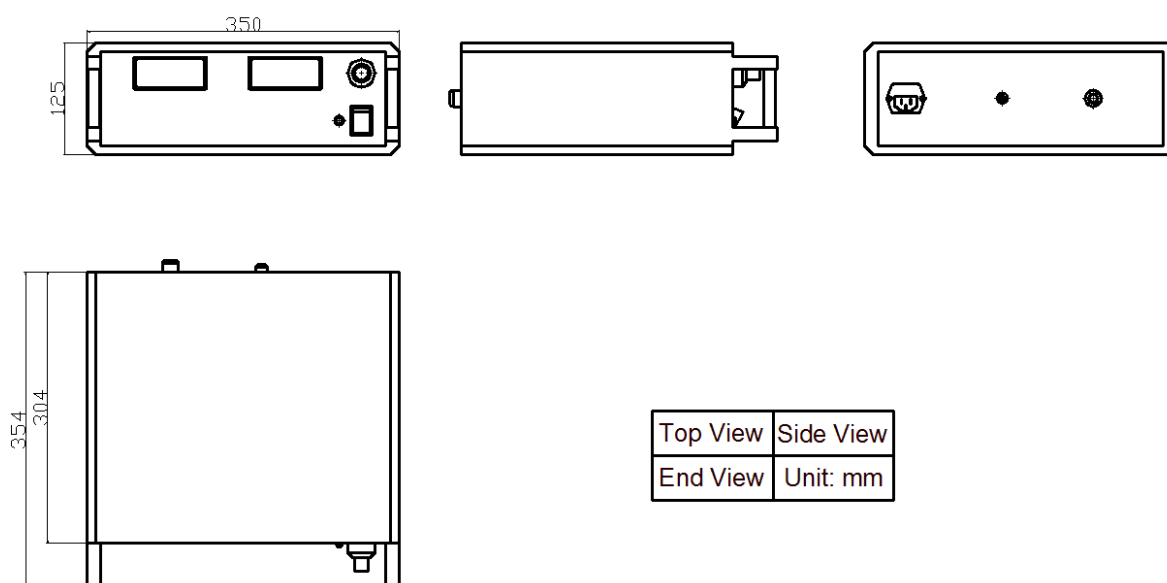
Figure 7. Dimensions for AHVAC50KVR5MABT
