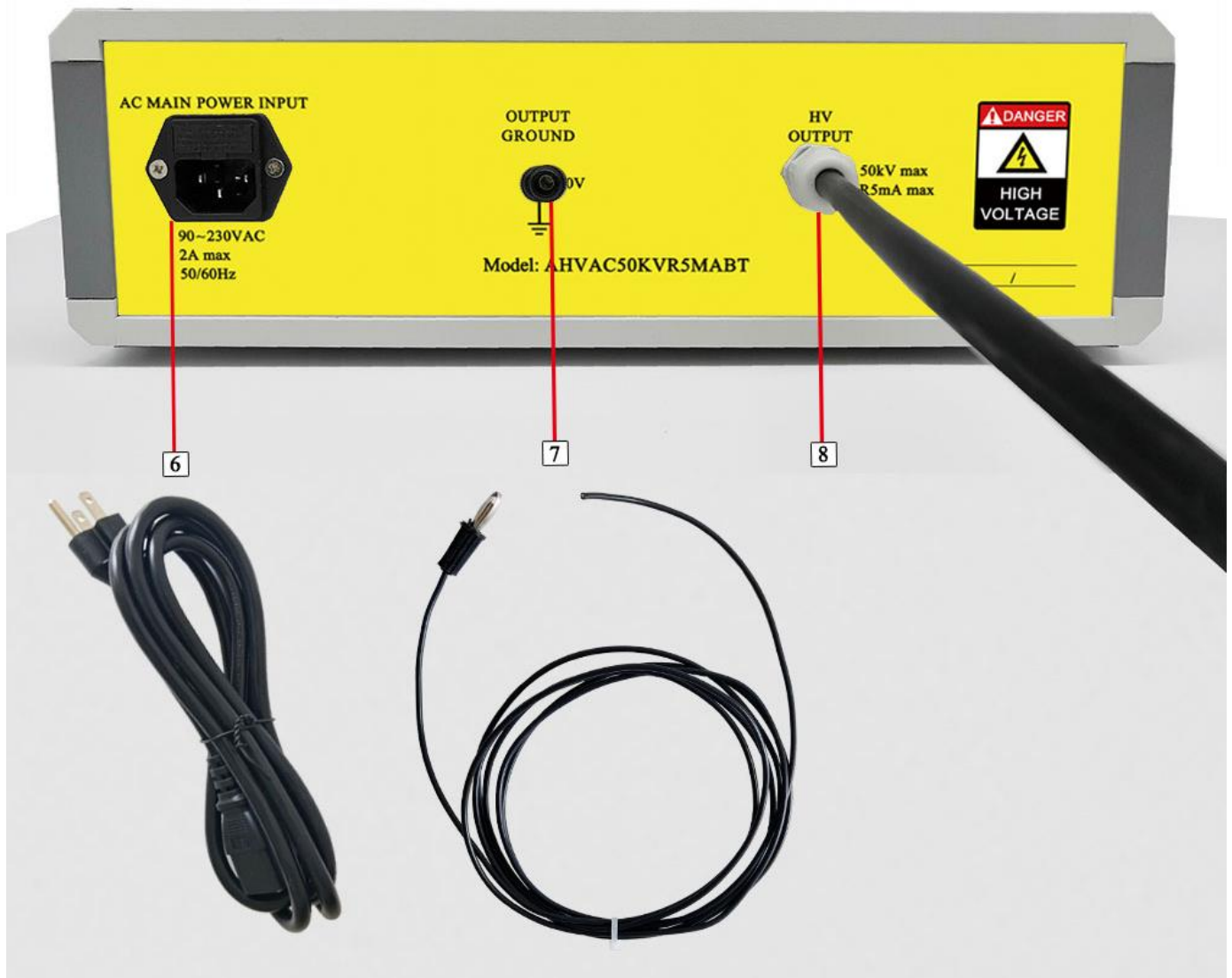
Figure 3. Back Panel
