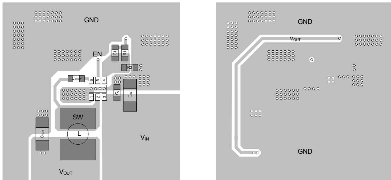
Figure 7. Suggested PCB
