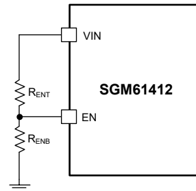
Figure 4. System UVLO by Enable Divider
