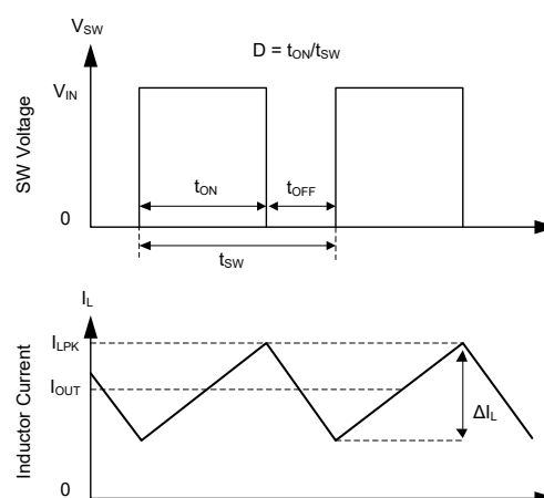
Figure 3. Converter Switching Waveforms in CCM
