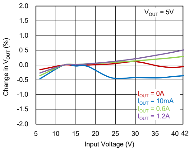
Line Regulation
