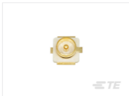
TE Part #CONUFL001-SMD-T U.FL/MHF1 Jack 50 Ohm PCB Surface Mount
