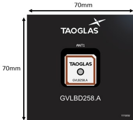
Top Side (70x70mm example PCB Reference Design)
