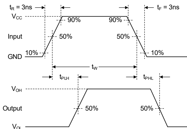
Figure 2. AC Waveforms
