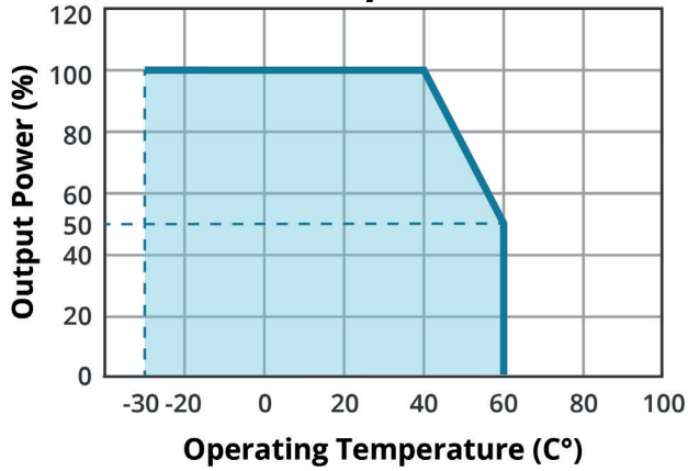
TEMPERATURE DERATING CURVE 5 Vdc output models
