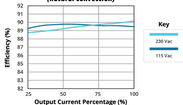
EFFICIENCY VS OUTPUT LOAD VOF-70B-24 (natural convection)
