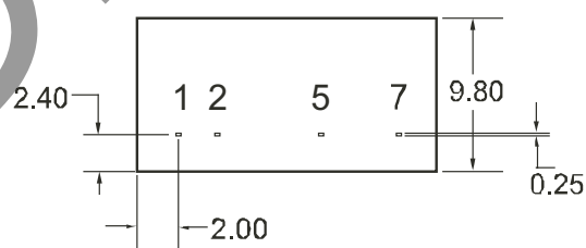
Bottom View
