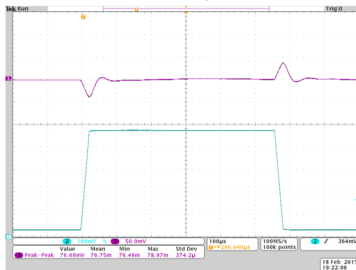
Transient Response
