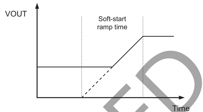
Illustration of Pre-Bias Startup.
