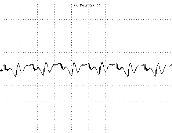
Figure 12: Output voltage ripple at nominal input voltage ( v_{in}=48\text{v} ) and rated load current ( I_o=10\text{A} ) (50 mV/div, 1 us/div). Load capacitance: 1\ \mu\text{F} ceramic capacitor and 100\ \mu\text{F} tantalum capacitor. Bandwidth: 20 MHz. Scope measurements should be made using a BNC cable (length shorter than 20 inches). Position the load between 51 mm to 76 mm (2 inches to 3 inches) from the module
