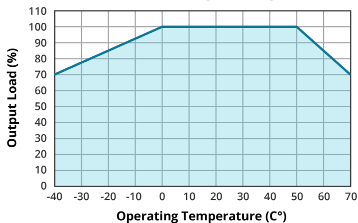
TEMPERATURE DERATING CURVE 12 & 15 Vdc output models (200~300 Vdc Input voltage)
