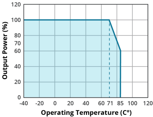
TEMPERATURE DERATING CURVE
