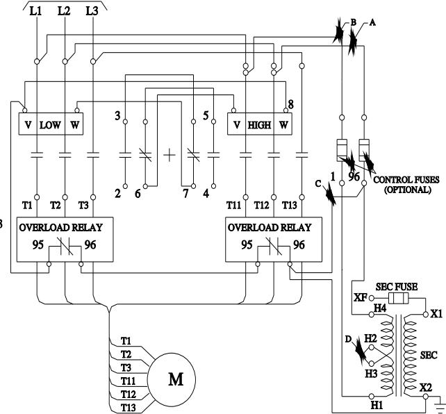
WIRING DIAGRAM
