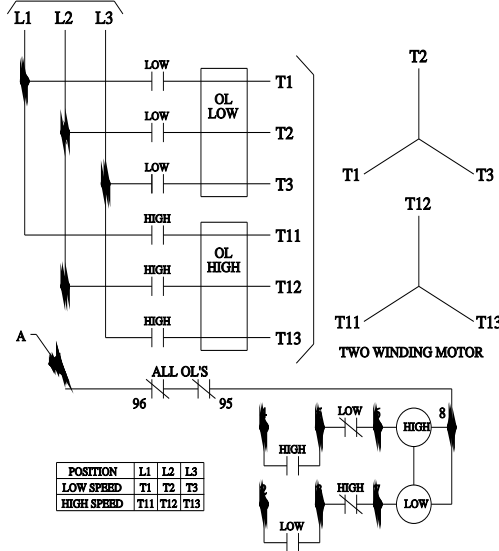
ELEMENTARY DIAGRAM
