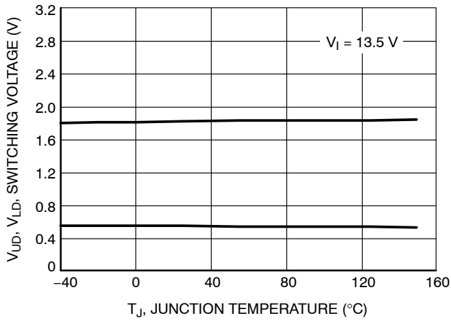
Figure 28. Switching Voltage vs. Junction Temperature
