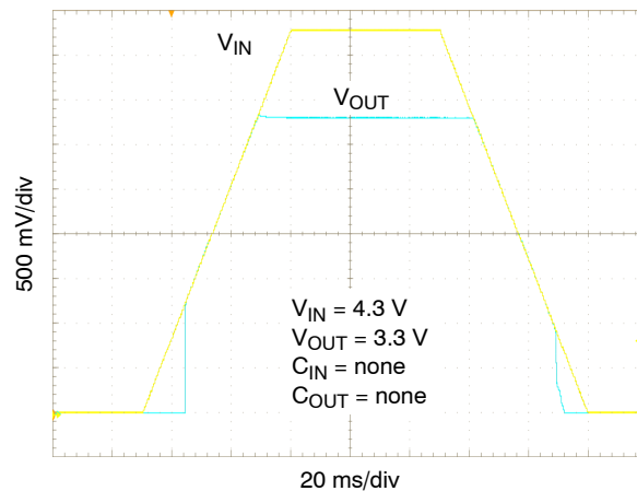
Figure 42. Slow V_{IN} Ramp
