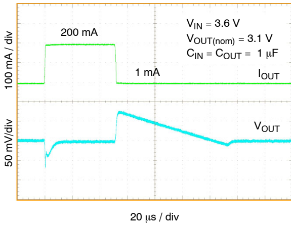
Figure 53. Load Transient Response I_{OUT} = 1\text{ mA to }200\text{ mA} , C_{OUT} = 1\text{ }\mu\text{F}
