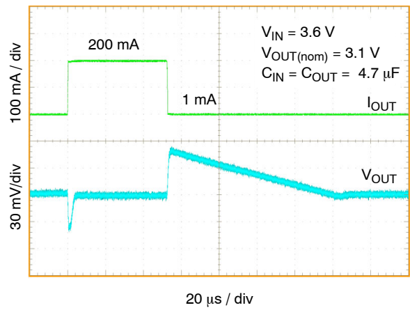
Figure 54. Load Transient Response I_{OUT} = 1\text{ mA to }200\text{ mA} , C_{OUT} = 4.7\text{ }\mu\text{F}
