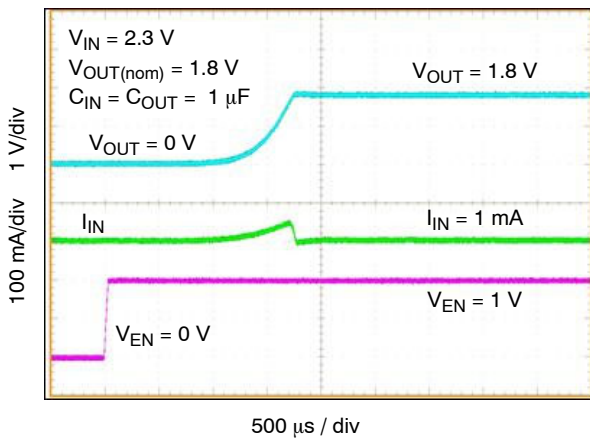
Figure 57. Enable Turn-On Response V_{OUT} = 1.8\text{ V} , C_{OUT} = 1\text{ }\mu\text{F}
