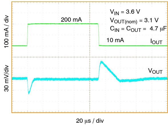
Figure 56. Load Transient Response I_{OUT} = 10\text{ mA to }200\text{ mA} , C_{OUT} = 4.7\text{ }\mu\text{F}
