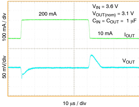
Figure 55. Load Transient Response I_{OUT} = 10\text{ mA to }200\text{ mA} , C_{OUT} = 1\text{ }\mu\text{F}
