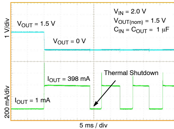
Figure 67. Short-Circuit Response V_{OUT} = 1.5 V, C_{OUT} = 1 \mu F
