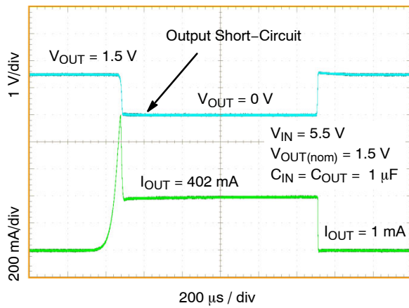
Figure 65. Short-Circuit Response V_{OUT} = 1.5 V, C_{OUT} = 1 \mu F
