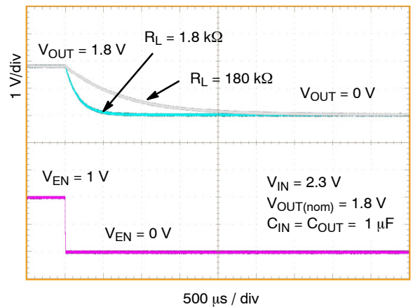
Figure 58. Enable Turn-Off Response V_{OUT} = 1.8\text{ V} , C_{OUT} = 1\text{ }\mu\text{F} (A Version)
