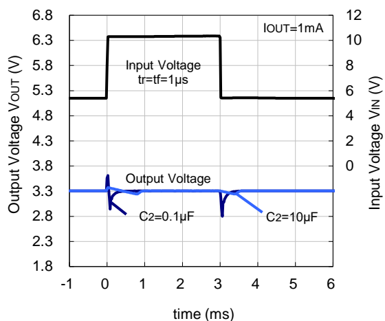
V SET = 3.3 V
