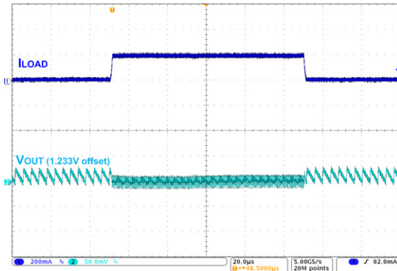
Figure 12. Load Transient, 10 mA ↔ 200 mA in 1 μs
