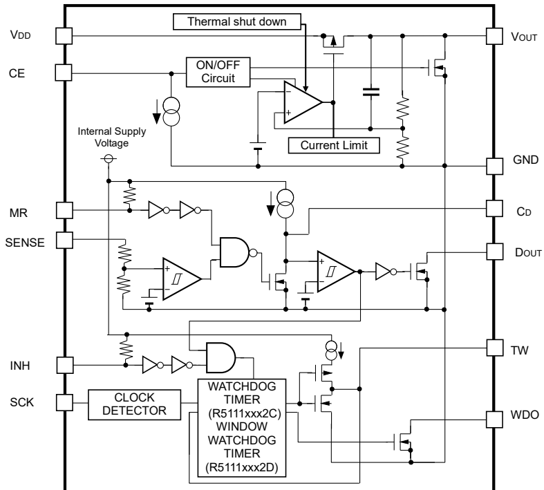
R5111xxx2C / R5111xxx2D
