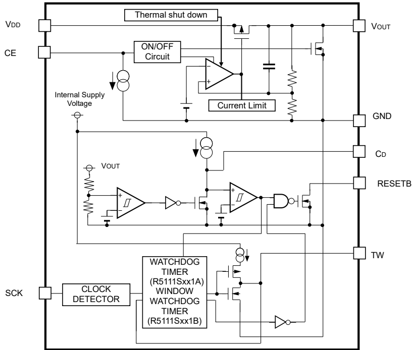
R5111Sxx1A / R5111Sxx1B
