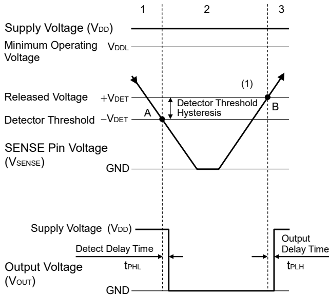
Operation Diagram
