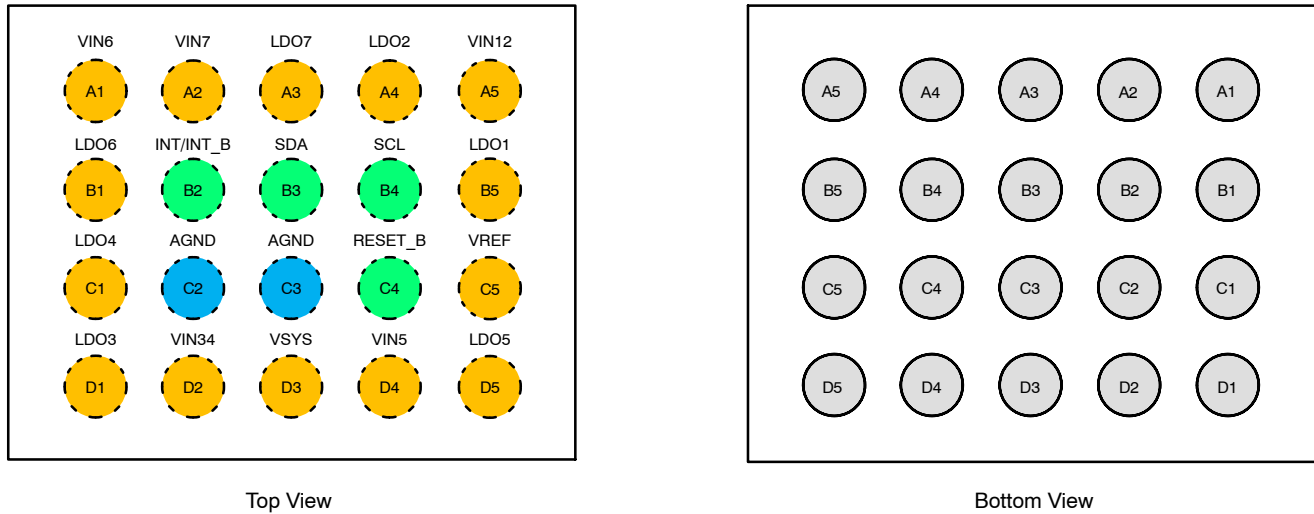
Figure 2. Pin Configuration
