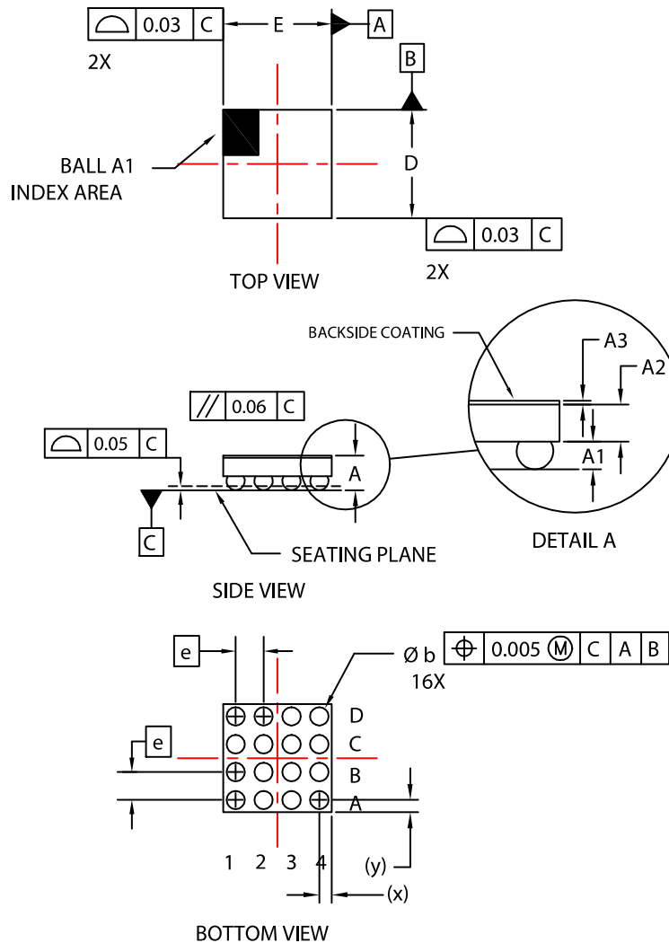
WLCSP16 1.52x1.52x0.432 CASE 567ZM ISSUE O
