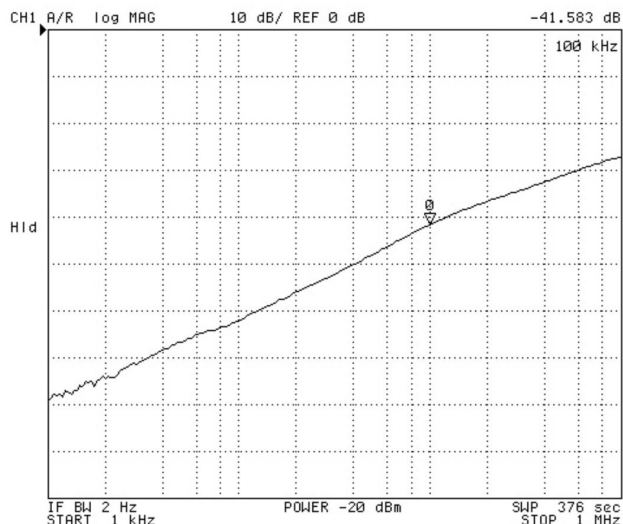
Figure 22. LDO3/4 PSRR vs. Frequency, V_{\text{OUT3/4}} = 1.8\text{ V} , I_{\text{OUT3/4}} = 100\text{ mA}
