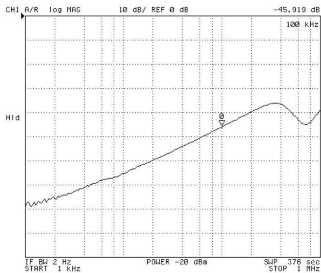
Figure 20. LDO1 PSRR vs. Frequency, V_{\text{OUT1}} = 1.05\text{ V} , I_{\text{OUT1}} = 150\text{ mA}
