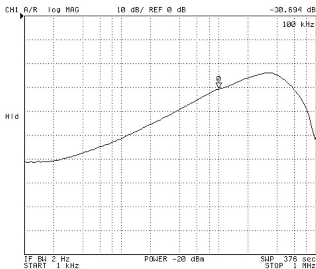
Figure 19. LDO1 PSRR vs. Frequency, V_{\text{OUT1}} = 1.2\text{ V} , I_{\text{OUT1}} = 150\text{ mA}
