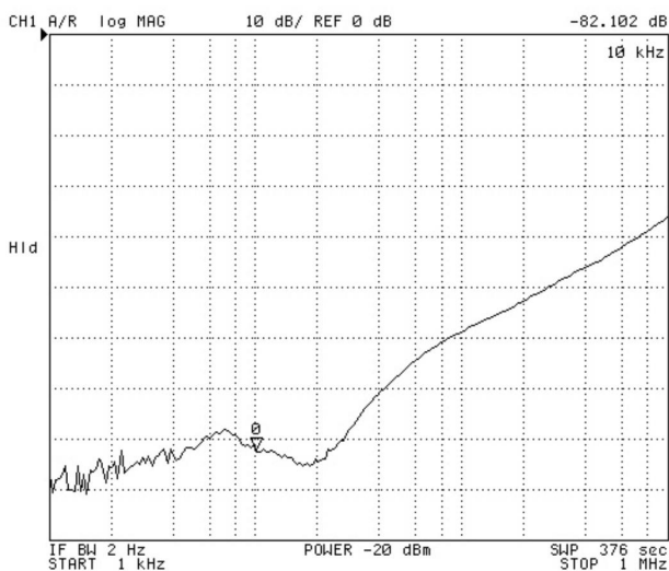
Figure 21. LDO2 PSRR vs. Frequency, V_{\text{OUT2}} = 2.85\text{ V} , I_{\text{OUT2}} = 100\text{ mA}
