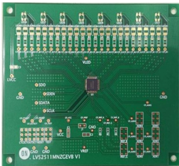
Figure 6. Board
