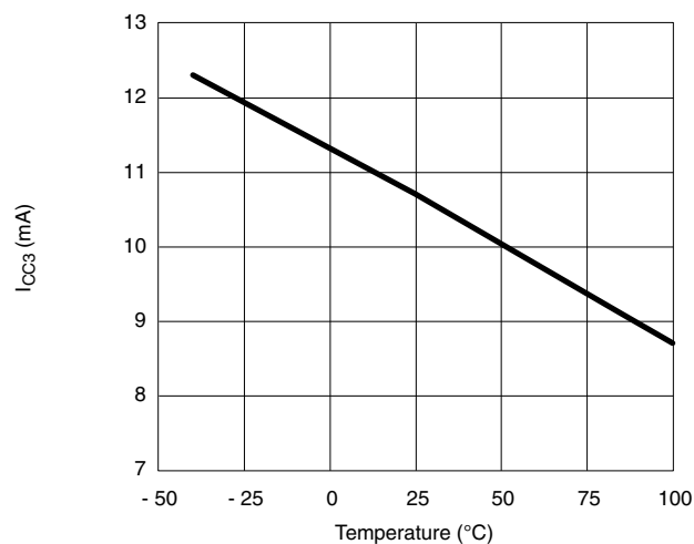
I_{CC3} vs. Temperature V_{CC} = 12 V
