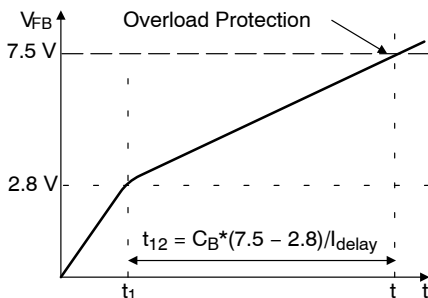
Figure 34. Overload Protection
