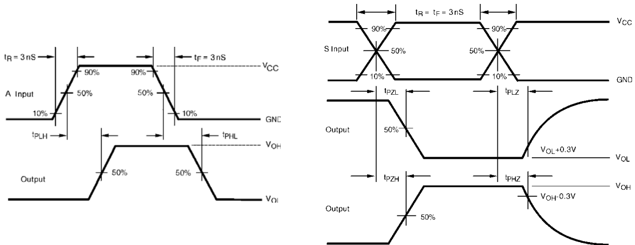
Figure 6. AC Waveforms
