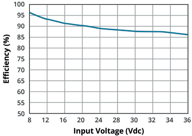
EFFICIENCY VS INPUT VOLTAGE (full load) V78E09-1000-SMT
