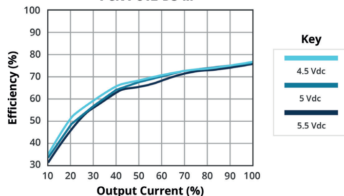
EFFICIENCY VS OUTPUT LOAD PCN1-S12-D5-M
