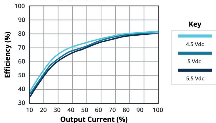
EFFICIENCY VS OUTPUT LOAD PCN1-S5-S12-M
