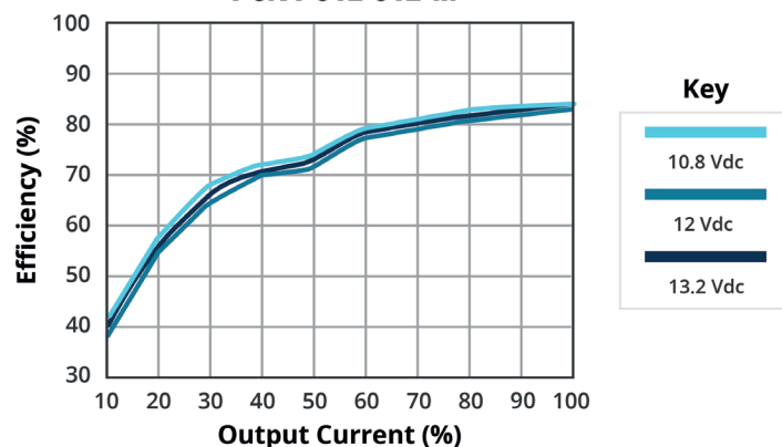
EFFICIENCY VS OUTPUT LOAD PCN1-S12-S12-M
