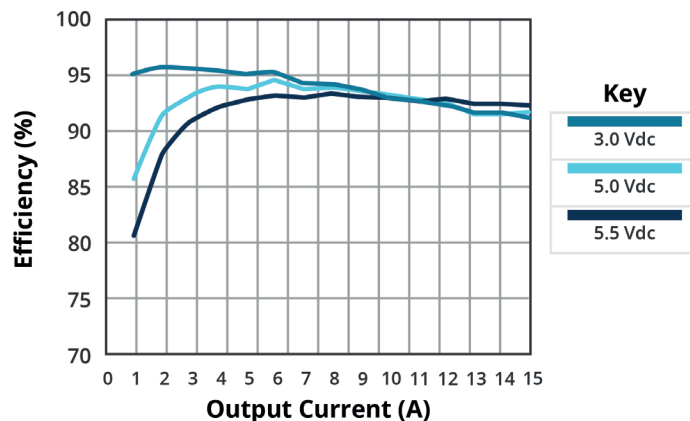
EFFICIENCY VS OUTPUT CURRENT VPOL15A-5-SMT ( V_o = 1.5 Vdc)
